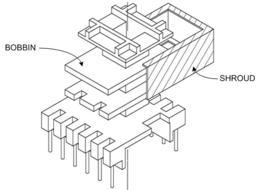
Figure 1. Vertical bobbin with shroud
